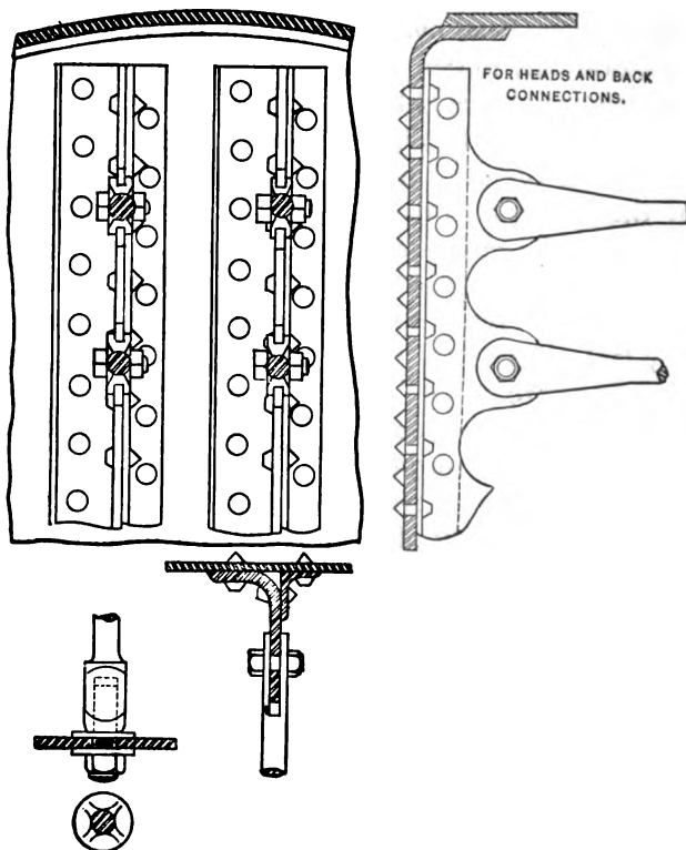
FIG. 107.—STAYING FLAT SURFACES.
